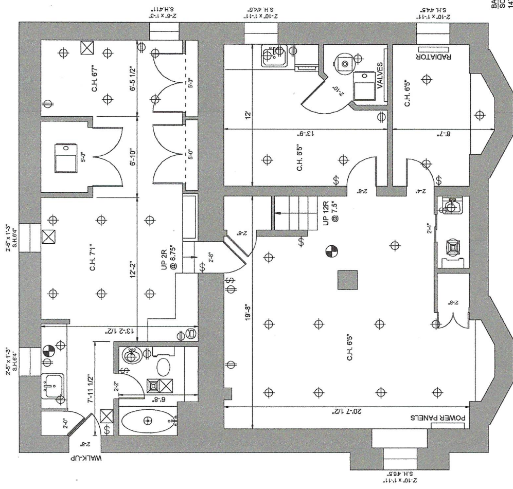
BASEMENT PLAN SCALE: 3/16" = 1' 1475 SQ. FT.
