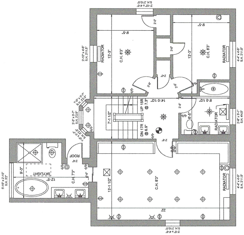
2nd FLOOR PLAN SCALE: 3/16" = 1' 1015 SQ. FT.
