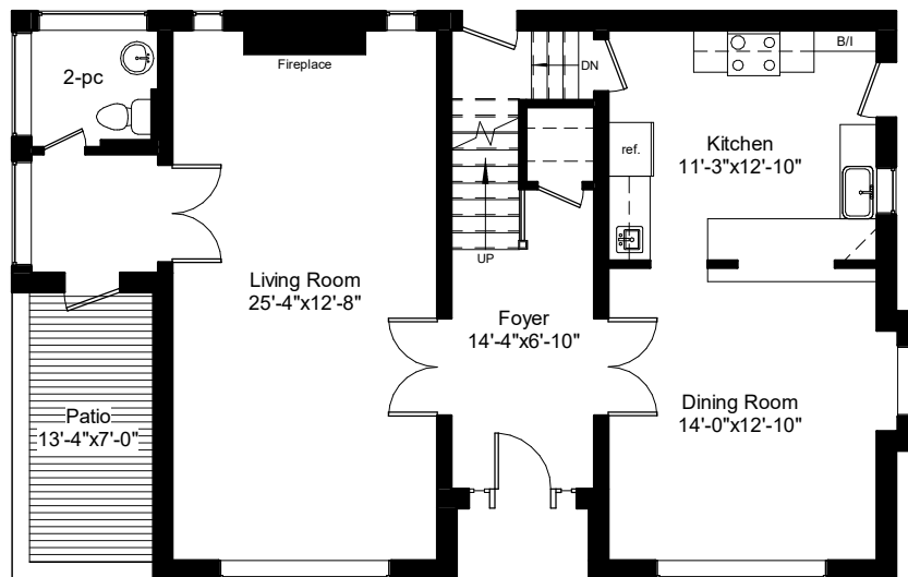
Main Level 1040 Square Feet
