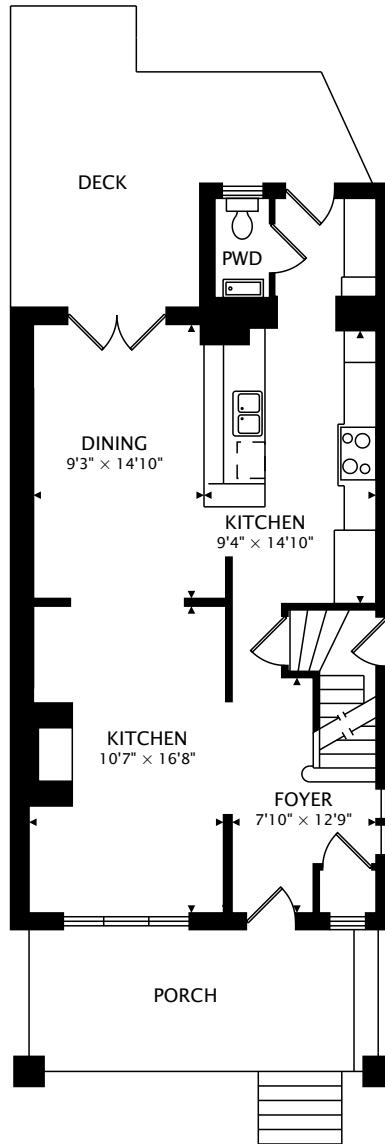
MAIN 777 sq ft
