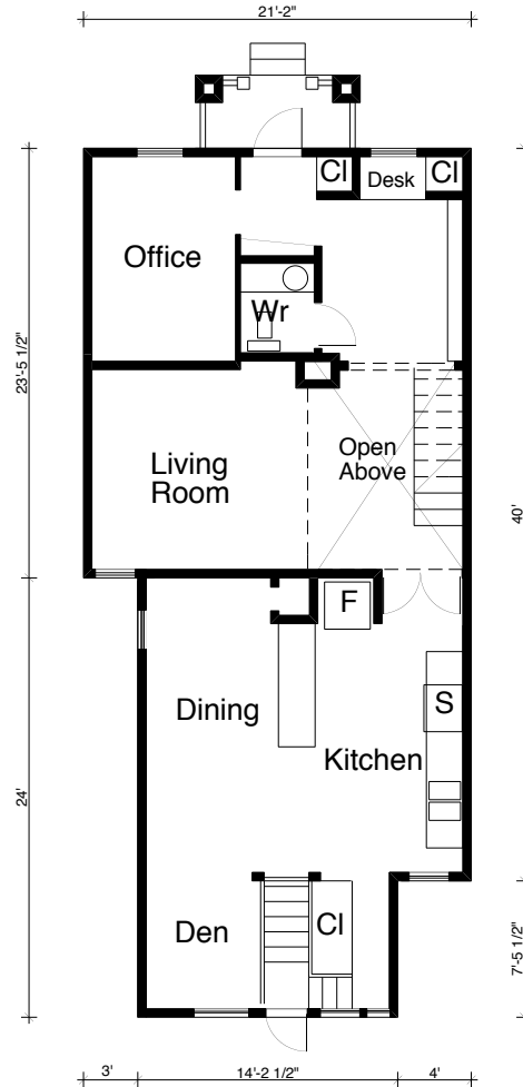
Ground Floor Plan 842 sq ft
