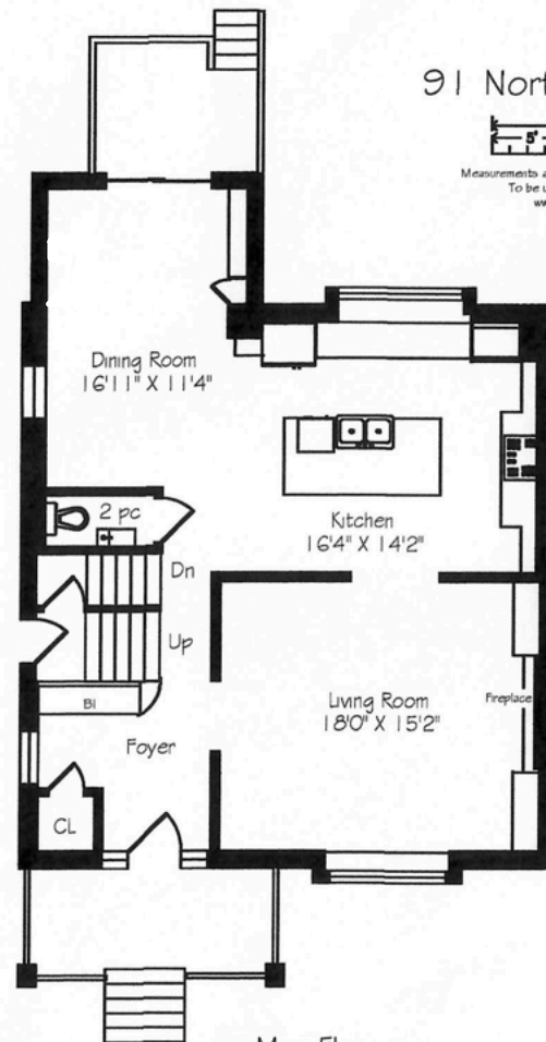
Main Floor 1077 Square Feet
